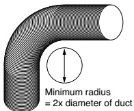
Figure 1. 90° bend
